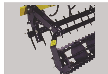
Spring loaded crumbler & spike bar
